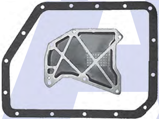
AISIN WARNER A210 (MX 17) DAIHATSU CHARADE 1988-1992 Pan Gasket A210.GAS01 Filter A210.FIL01
