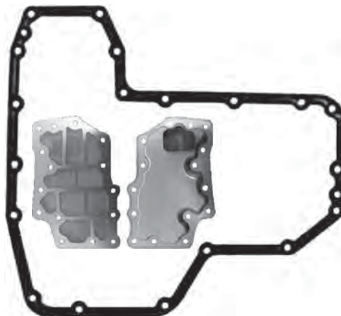
JATCO JF009E, NISSAN REOF08A (NISSAN CUBE, MICRA, TIDA & WINGROAD) Pan Gasket TBA Filter TBA
