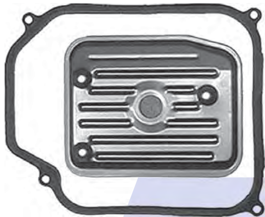
01M (VW 4 SPEED FWD) Pan Gasket AD4.GAS01 Filter AG4.FIL03
