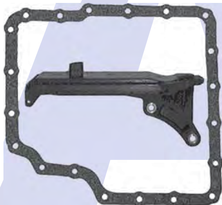
09A (JF506E) AUDI A3 Pan Gasket JF506E.GAS01 Filter JF506E.FIL13 Pick Up 17mm Angled
