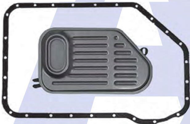
01V (5HP19FL) 2WD CODE 1060 030 XXX Pan Gasket 5HP19.GAS03 Filter 5HP19.FIL02 Pick Up 8mm High
