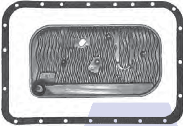
ALLISON AT-540 Pan Gasket AT545.GAS01 Filter AT545.FIL01
