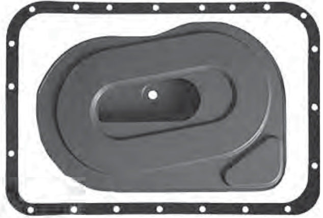
ALLISON AT-640 Pan Gasket AT545.GAS01 Filter AT545.FIL02
