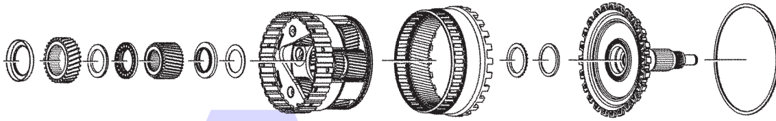
904 Rear Planetary and Output
