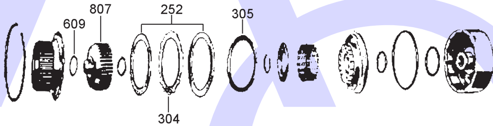
Forward Clutch
