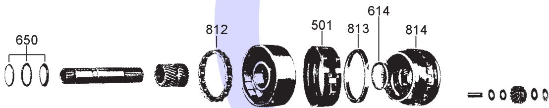
Forward Clutch
