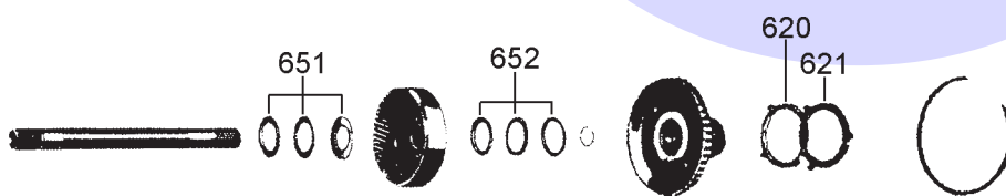
Sun Gear, Low/Reverse Band & Planetary
