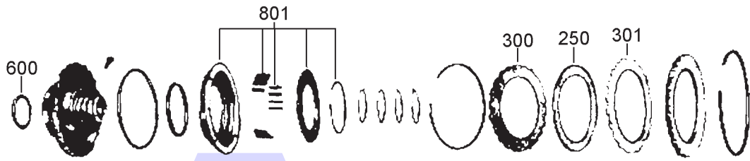
Centre Support
