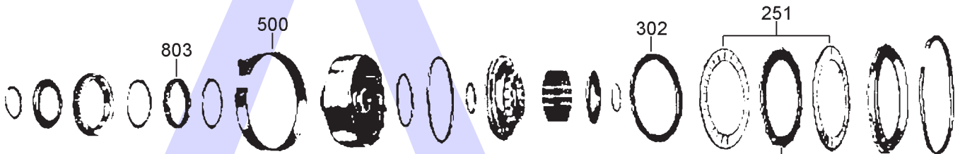
Centre Support
