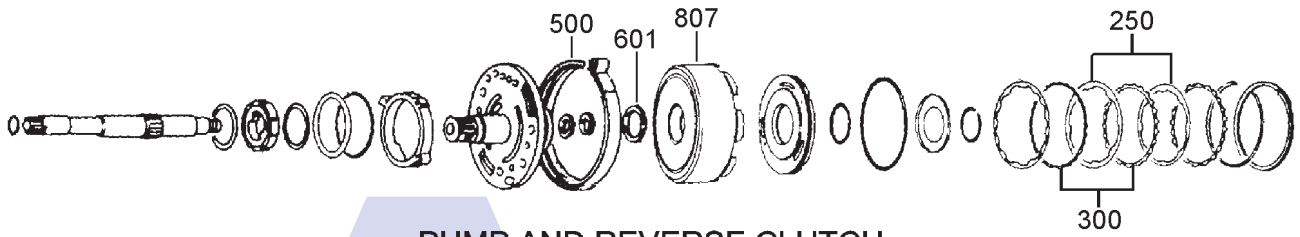
PUMP AND REVERSE CLUTCH
