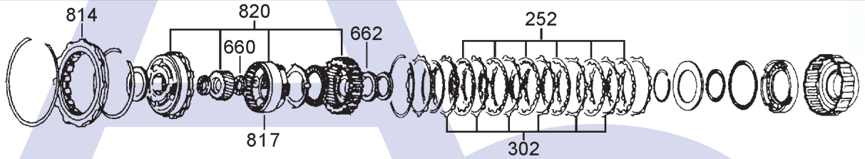
PLANET SET AND LOW CLUTCH
