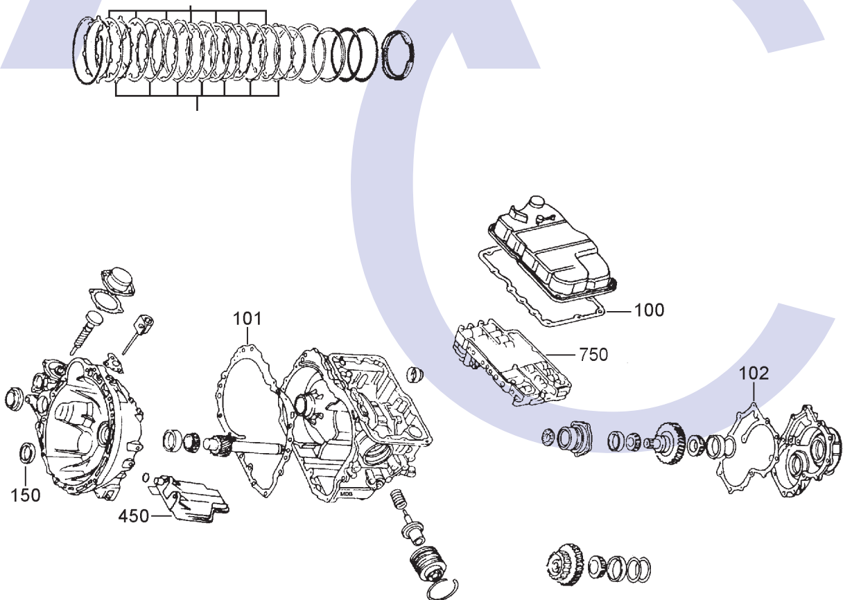
LOW REVERSE CLUTCH AND CASE
