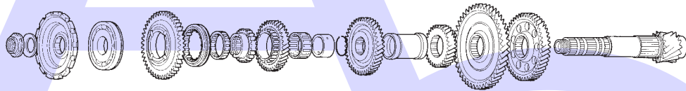
Countershaft
