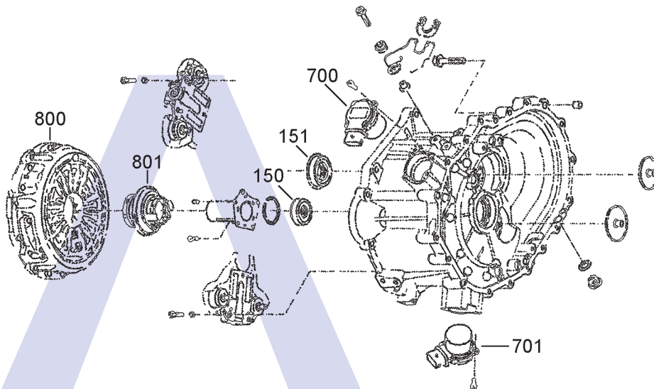
Clutch, Clutch Control and Bell Housing
