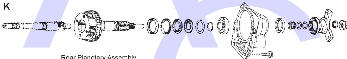
Rear Planetary Assembly
