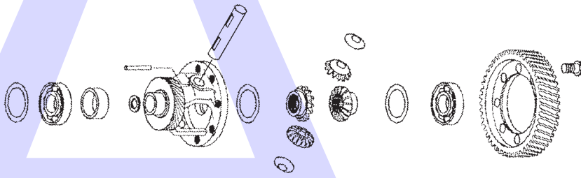
Differential Assembly
