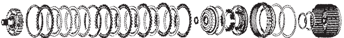
Reverse & Overdrive Clutch
