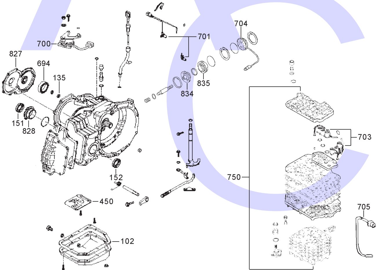
Main Case, Oil Pan, Filter, Valve Body & External Components
