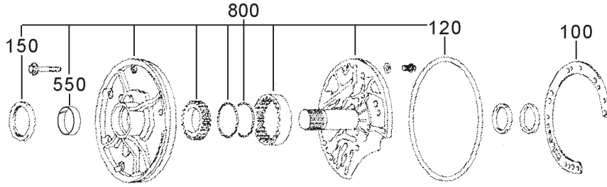
Oil Pump Assembly
