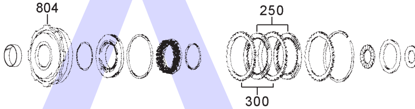
Direct Clutch Assembly
